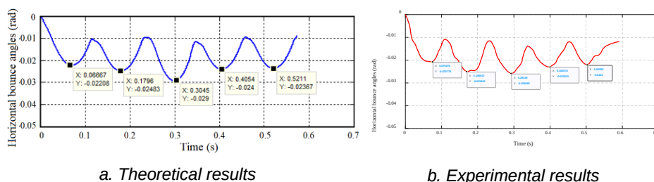
Figure 18 – The barrel's bounce angle in the horizontal plane when firing bursts of five rounds
