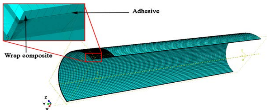
Figure 3 - Mesh representation of the repair zone, including the composite overwrap and adhesive layer. Refined meshing in these areas ensures accurate stress transfer between materials with differing stiffnesses
