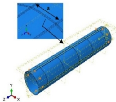
Figure 10 - Boundary conditions for a pipeline with a circumferential crack subjected to compressive forces ( U < 0 )
