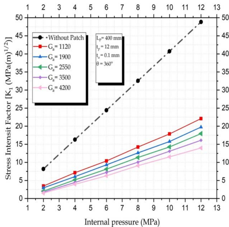
Figure 9 - Variation of Stress Intensity Factor (SIF) with Internal Pressure for Various Adhesive Shear Moduli
