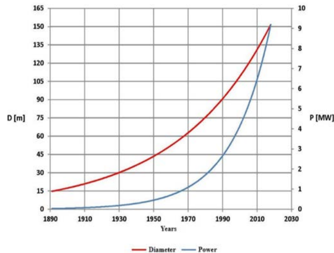
Figure 2 - Trend in the increase of rotor diameter and wind turbine power (Hossain et al, 2018)
