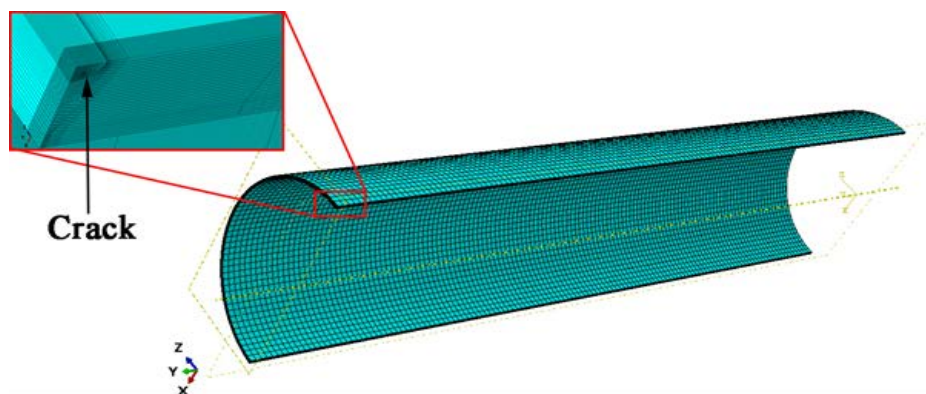
Figure 2 - Global view of the finite element mesh of the cracked pipeline, with a zoom on the surface crack region. Local mesh refinement enables accurate capture of stress singularities at the crack front
