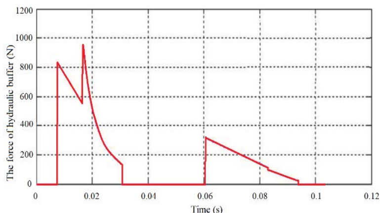
Figure 5 – The braking force of the hydraulic buffer
