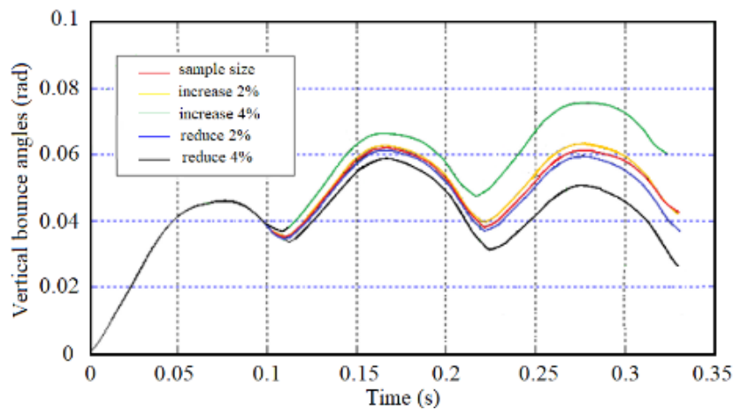
Figure 24 – The barrel's bounce angle in the vertical plane
