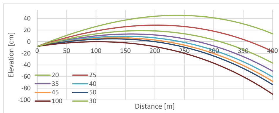
Figure 5 - Bullet flight path
