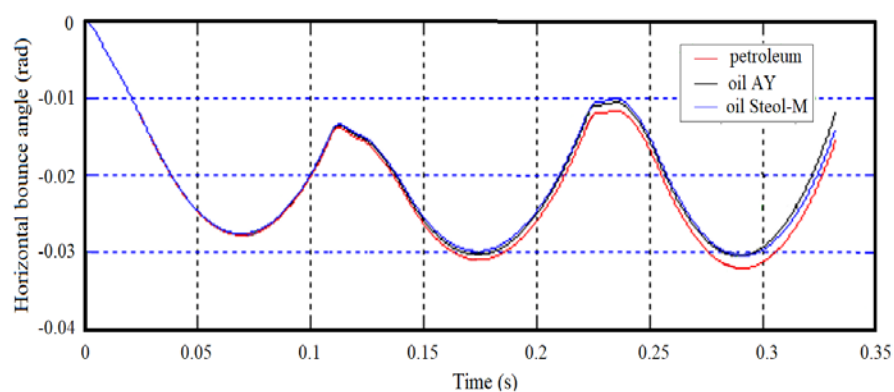
Figure 22 – The barrel's bounce angle in the horizontal plane when firing bursts of three rounds
