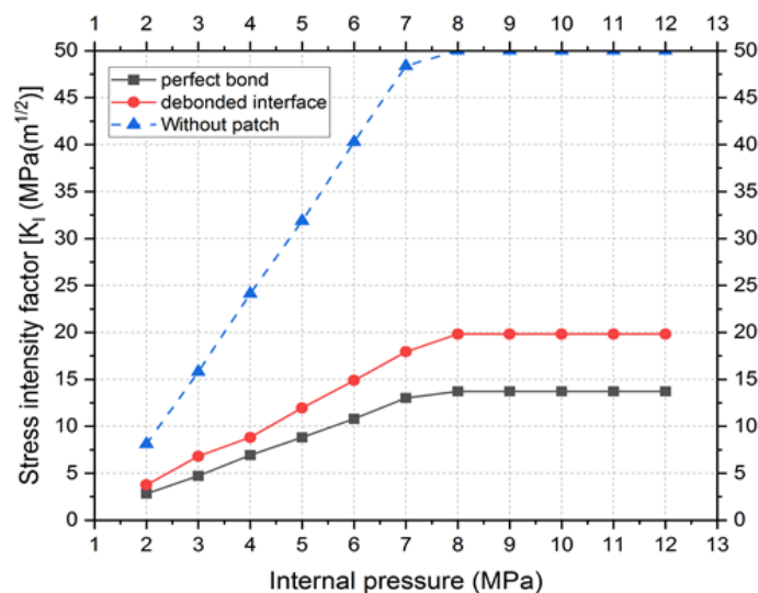
Figure 11 - Impact of Adhesive Debonding on Stress Intensity Factor
