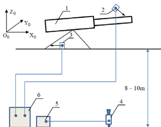
Figure 9 – Experimental diagram: 1. Gun; 2,3. Displacement measuring device; 4. High-speed camera; 5. Computer; 6. DEWETRON 3000 device.
