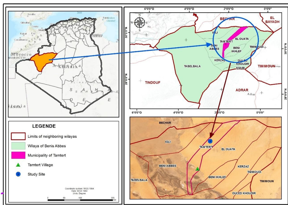
Figure 1 – Geographical location of the Tamtert region (Malti, 2012)
