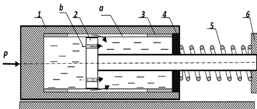
Figure 3 – Working principle model of hydraulic buffer mechanism 1. Bolt; 2. Piston; 3. Regulating tube; Sealing Parts; 5. Return spring; 6. Gun body; a - Oil drain; b - Oil drain hole
