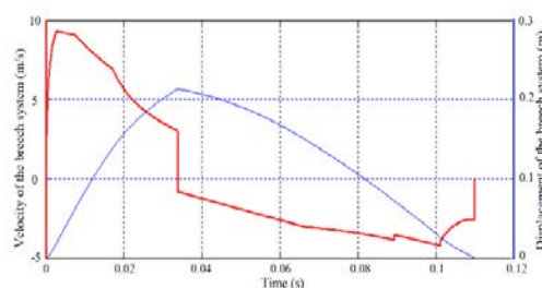
Figure 14 – Velocity and displacement of the bolt with time
