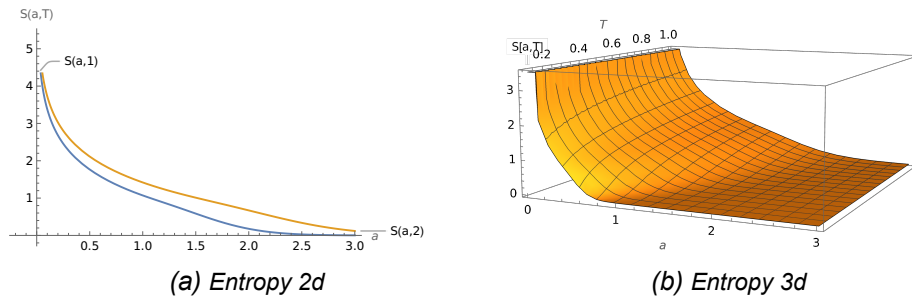
Figure 6 – Entropy as a function of a and T
