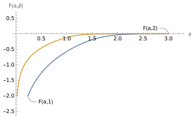
Figure 4 – Free energy F(a, \beta) as a function of energy parameter a for different values of \beta
