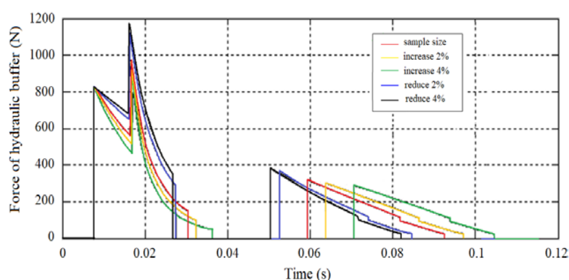
Figure 23 – Hydraulic braking force with different oil flow area
