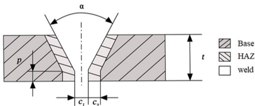
Figure 1 - Schematic representation of the circumferential welded joint geometry
