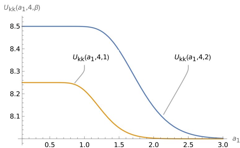
Figure 9 – Internal energy U^{KK}(a_1, a_2, \beta) of toy KK model as a function of energy parameter a_1 and fixed a_2 for different values of \beta
