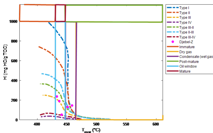
Figure 6 – Cross plot of (HI) versus (Tmax) for Djebel-Zereg samples. Reproduced from (Hong et al., 2021)
