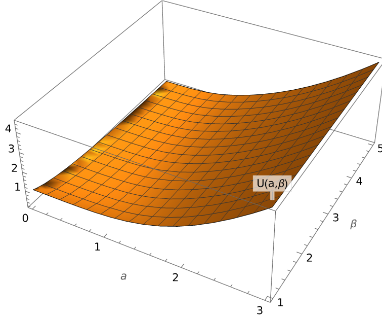
Figure 8 – Internal energy U^{ho}(a, \beta) of harmonic oscillator as a function of energy parameter a and \beta
