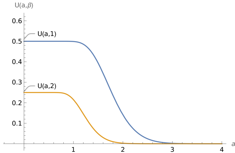
Figure 1 – Internal energy U(a, \beta) as a function of energy parameter a for different values of \beta
