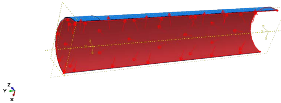
Figure 4 - Application of internal pressure on the internal surface of the quarter-cylinder pipe model
