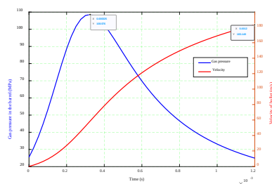
Figure 13 – Combustion gas pressure and bullet velocity in the barrel
