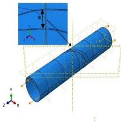
Figure 16 - Boundary conditions for a pipeline containing a crack oriented at 45° subjected to tensile forces ( U > 0 )
