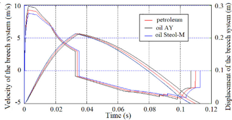
Figure 20 – Velocity and displacement of the bolt
