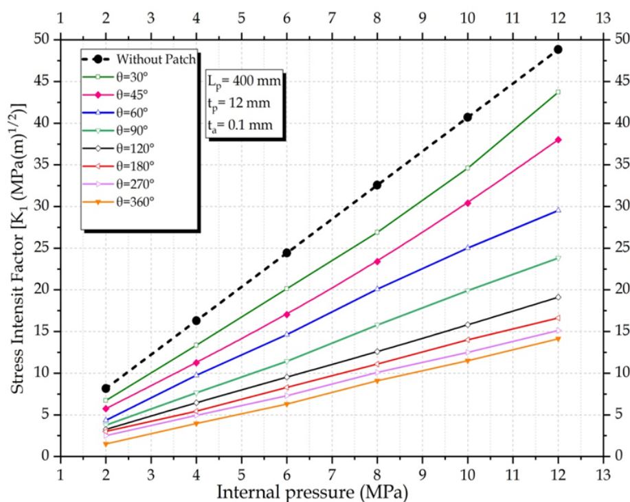
Figure 8 - Variation of SIF with Internal Pressure for Different Wrap Coverage Angles
