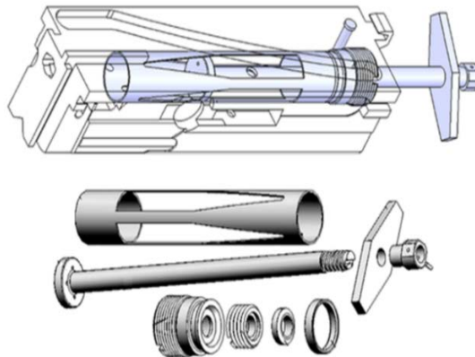
Figure 2 – Hydraulic buffer mechanism
