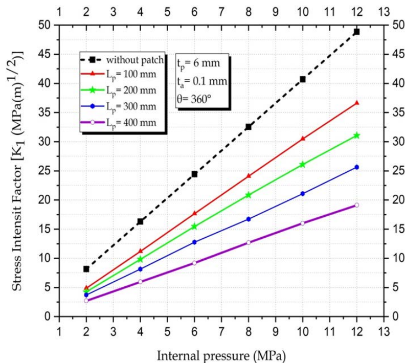
Figure 6 - Variation of SIF with Internal Pressure for Various Wrap Lengths
