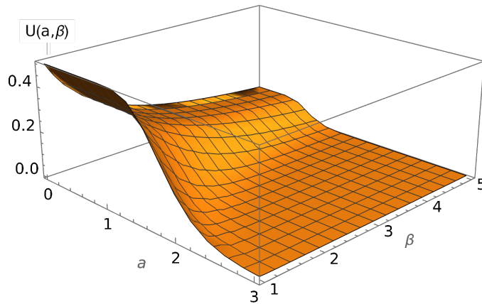
Figure 2 – Internal energy U(a, \beta) as a function of a and \beta
