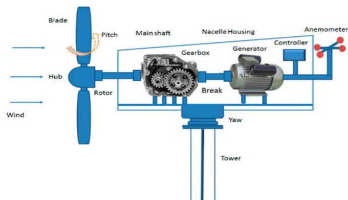
Figure 1 – Wind Turbine System (Gao & Liu, 2021)
