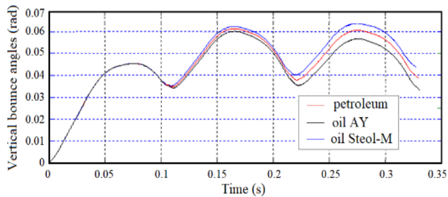
Figure 21 – The barrel's bounce angle in the vertical plane when firing bursts of three rounds
