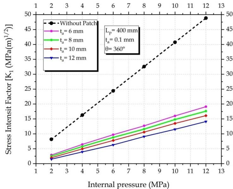
Figure 7 - Variation of SIF with Internal Pressure for Different Wrap Thicknesses
