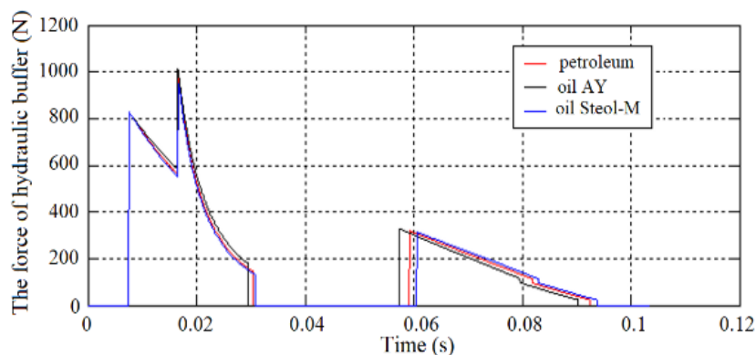
Figure 19 – Force of hydraulic buffer
