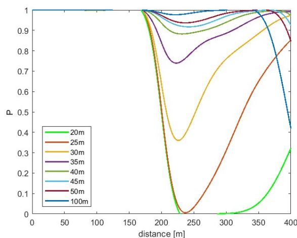
Figure 6 - Hit probability (prone, E-type) with aim point shift at 200 m
