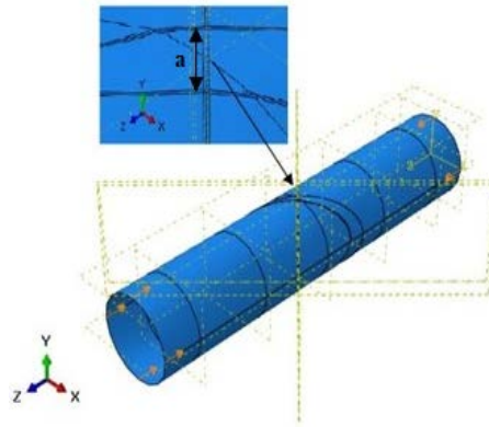
Figure 17 - Boundary conditions for a pipeline containing a crack oriented at 45° subjected to compressive forces ( U < 0 )
