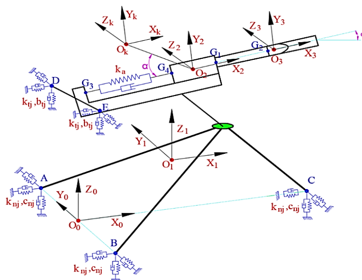
Figure 6 – Automatic gun model mounted on the tripod (Bien et al, 2021)
