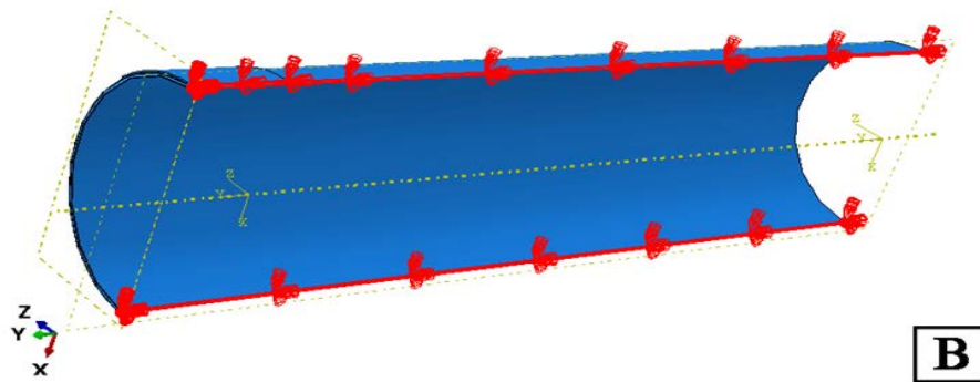
Figure 5 - Boundary conditions applied to the repaired pipeline model – (A) Longitudinal symmetry plane ( U_Y = \theta_X = \theta_Z = 0 ); (B) Circumferential symmetry plane ( U_Z = \theta_X = \theta_Y = 0 )
