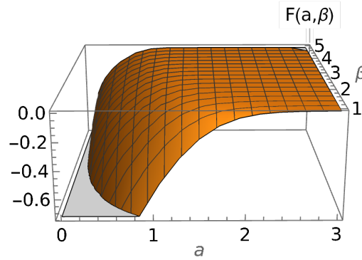
Figure 5 – Free energy F(a, \beta) as a function of a and \beta
