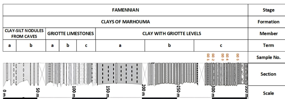
Figure 2 – Modified lithostratigraphic columnar section of 'Argiles de Marhouma' Formation in Saoura Valley (Tamtert-Zereg). Reproduced from (Malti, 2012)
