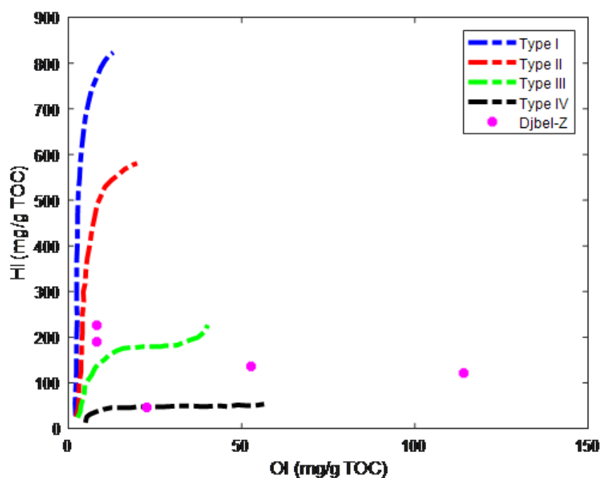
Figure 5 – Cross plot of HI versus OI for Djebel-Zereg samples. Reproduced from (Akinwumiju & Satterfield, 2024)
