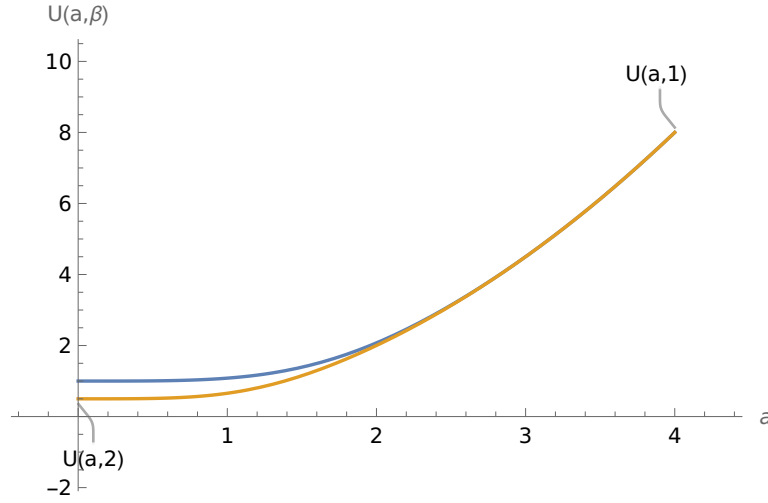
Figure 7 – Internal energy U^{ho}(a, \beta) of harmonic oscillator as a function of energy parameter a for different values of \beta
