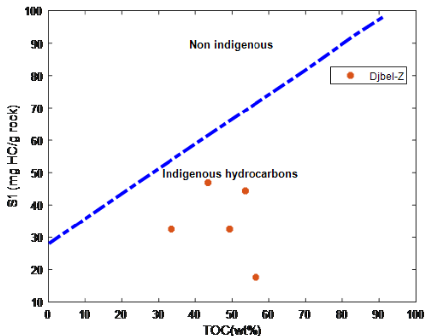
Figure 4 – Cross plot of S1 versus TOC for Djebel-Zereg samples. Reproduced from (Edress et al., 2022)
