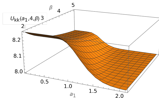
Figure 10 – Internal energy U^{KK}(a_1, a_2, \beta) of toy KK model as a function of energy parameter a_1 and fixed a_2 for different values of \beta
