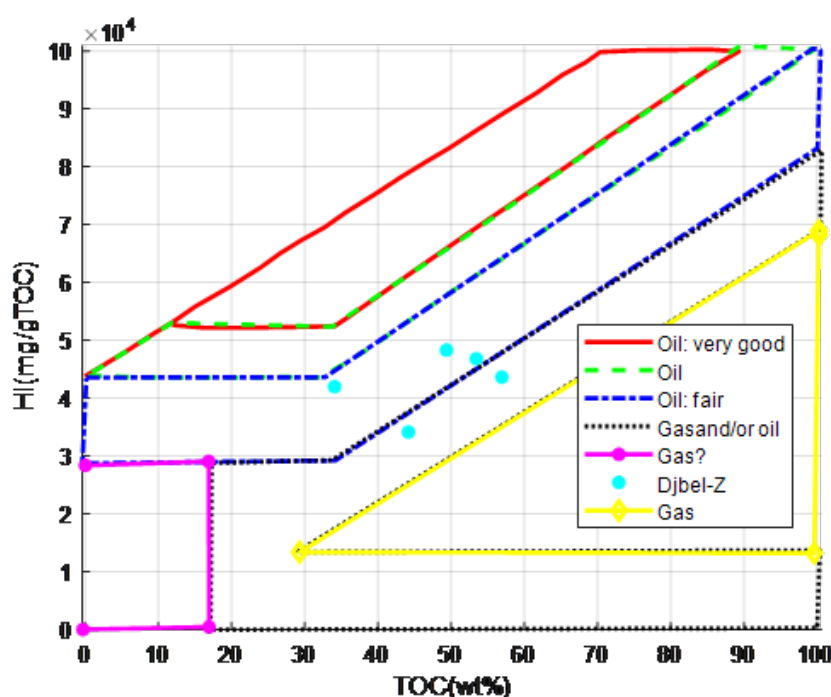
Figure 3 – Cross plot of HI versus TOC for Djebel-Zereg samples. Reproduced from (Sohail et al., 2024)
