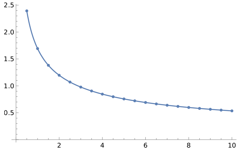
Figure 3 – Fit for critical values of a as function of \beta
