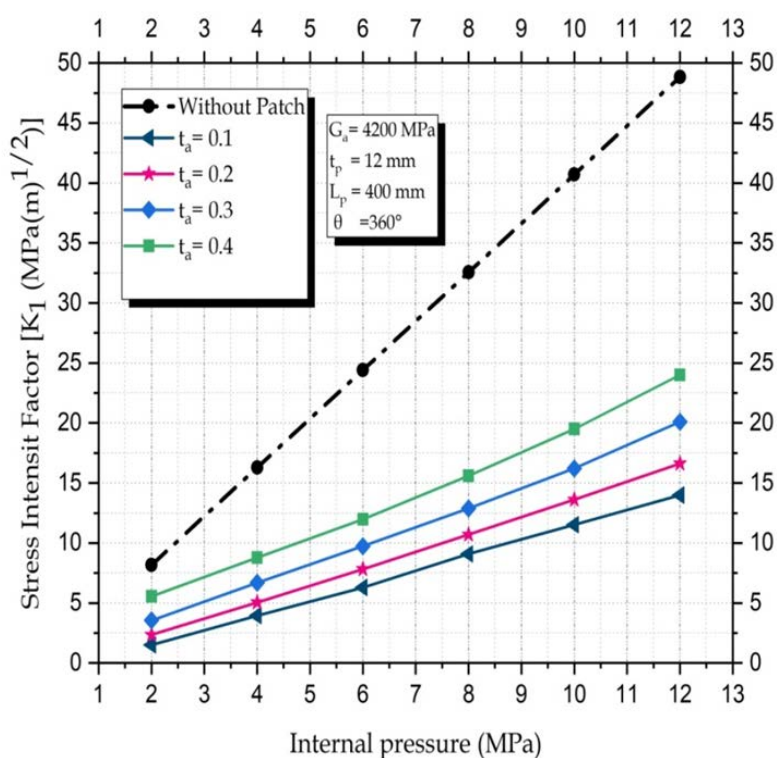
Figure 10 - SIF vs. internal pressure for different thickness of adhesive
