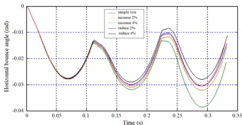
Figure 25 – The barrel's bounce angle in the horizontal plane
