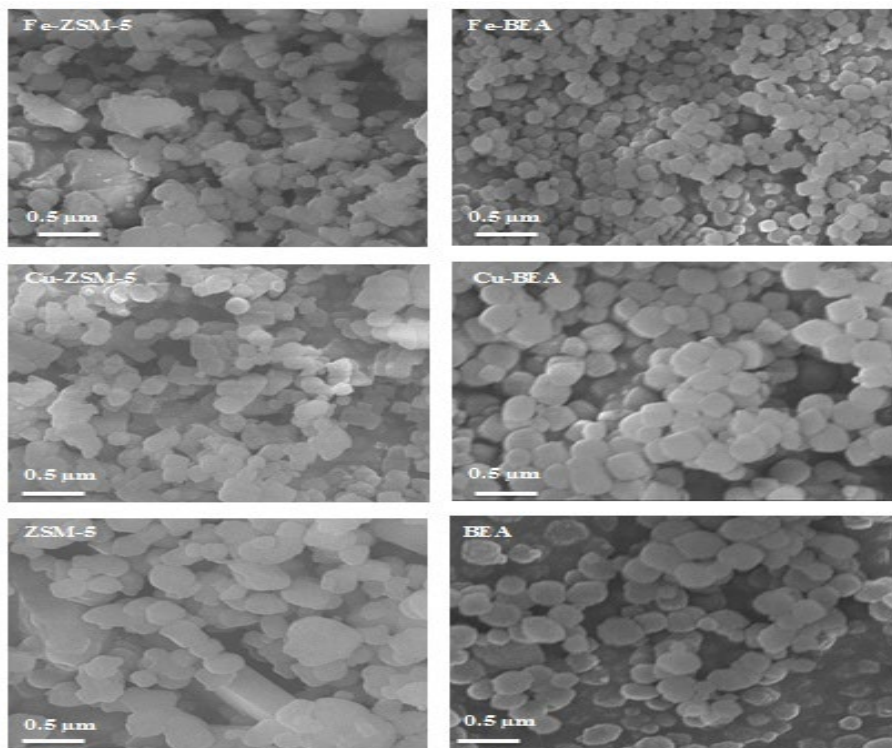
Figure 3- Scanning electron microscopy (SEM) images of BEA, Cu-BEA, Fe-BEA, ZSM-5, Cu-ZSM-5, and Fe-ZSM-5
