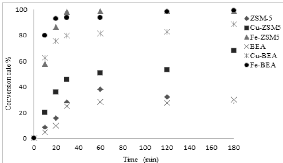
Figure 6 - Conversion of phenol as a function of time on pure catalysts and M + -zeolite catalysts ( T = 80^{\circ}C , C_{cPh} = 0.01 \text{ mol/l} , C_{c H_2O_2} = 0.10 \text{ mol/l} , m_{cat} = 0.10 \text{ g/l} , and pH = 4.2 )
