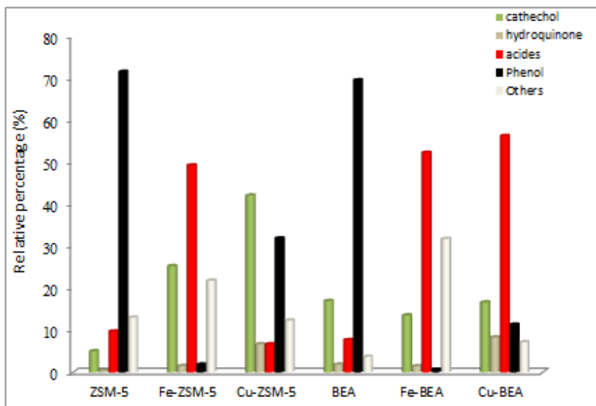
Figure 5-Distribution of by-products on catalysts based on M^{+}/\text{zeolites} ( T = 80^{\circ}\text{C} , C_c \text{ Ph} = 0.01 \text{ mol/l} , C_c \text{ H}_2\text{O}_2 = 0.10 \text{ mol/l} , m_{\text{cat}} = 0.10 \text{ g/l} , and \text{pH} = 4.2 )
