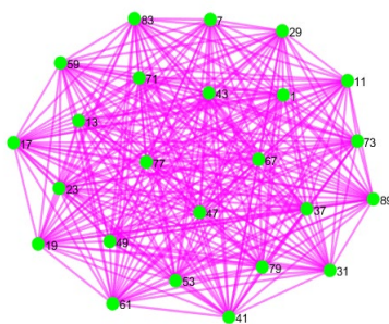
Figure 1 – Graph for G_2(Z_{90})
