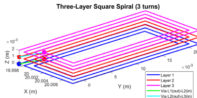
(b) 3-layer rectangular planar coil
