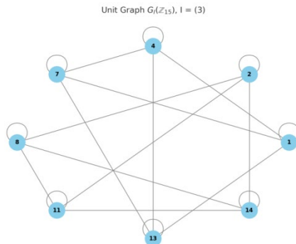
Figure 8 - Unit graph of G_3(Z_{15})
