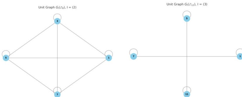
Figure 7 - Unit graphs of G_2(Z_8) and G_3(Z_{12})
