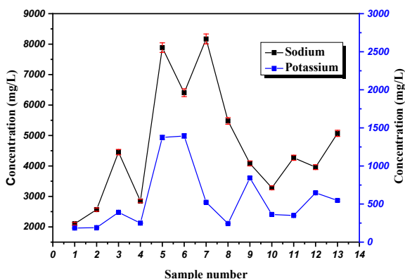
Figure 7 – Curve of the sodium and potassium ion content monitoring in the unhairing wastewater from the tannery, the Batna Unit
