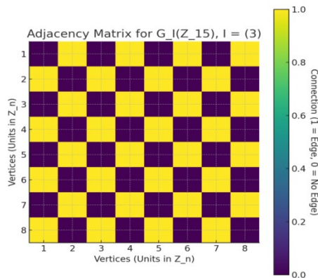
Figure 10 - Heat map of the adjacency matrix for G_3(Z_{15})
