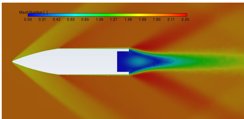
Figure 11 - Mach number profile around the projectile with the base cavity afterbody at Mach 2.0
