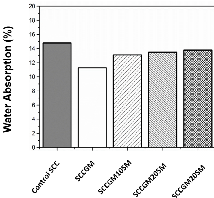
Figure 11 – Water absorption as a function of SCC with RMA (source author)
