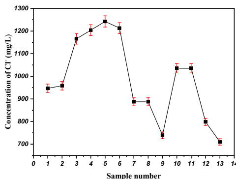
Figure 8 – Curve of the chloride ion content monitoring in the unhairing wastewater from the tannery, the Batna Unit
