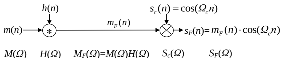
Figure 14 – Discrete-filtered pulse modulator
