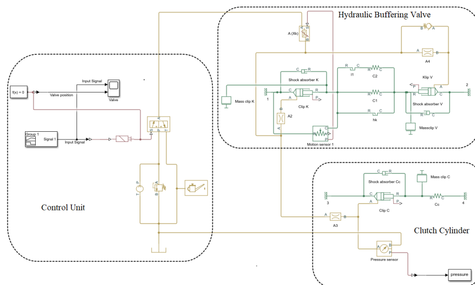
Figure 4 – Simulation model of the hydraulic buffering valve
