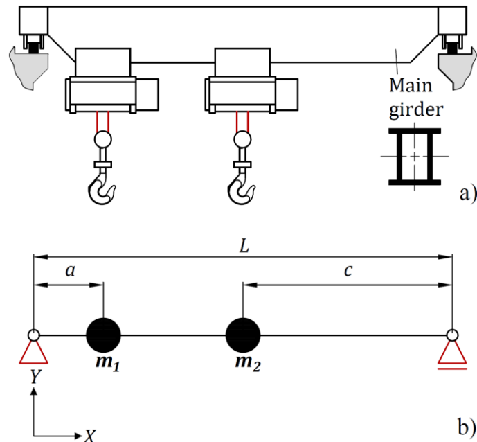
Figure 3 – a) Sketch of a bridge crane with two winches, b) Model with the concentrated masses of the carrying structure of the bridge crane
