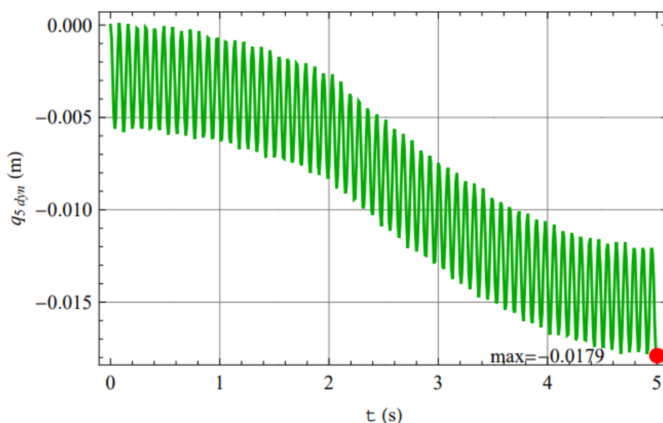
Figure 9 – Response – displacement, node 5 - q_{5dyn}
