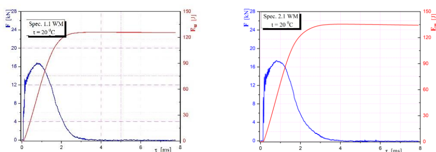
Figure 5 – Diagrams of the impact tests of the test specimens from experimental plates 1 and 2 with a notch in the filler metal
