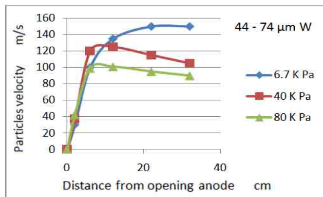
Figure 6 – Average velocities of W particles with a granulation of 44-74 \mu\text{m} with the change of pressure
