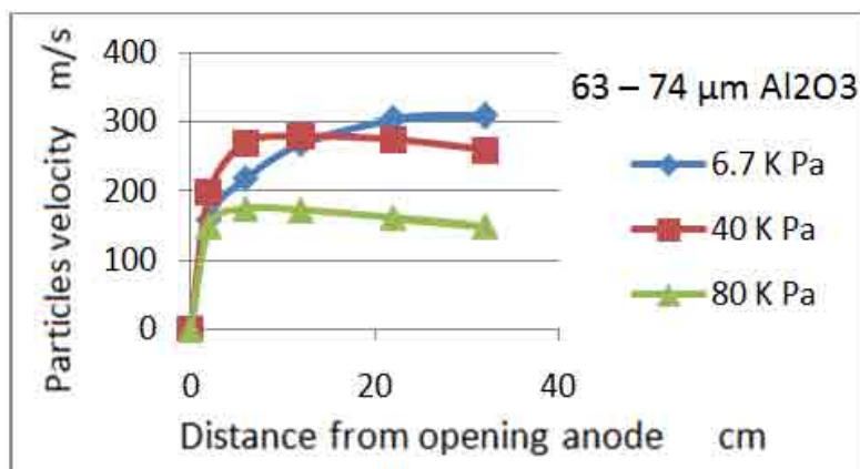
Figure 5 – Average velocities of \text{Al}_2\text{O}_3 particles with a granulation of 63-74 \mu\text{m} with the change of pressure
