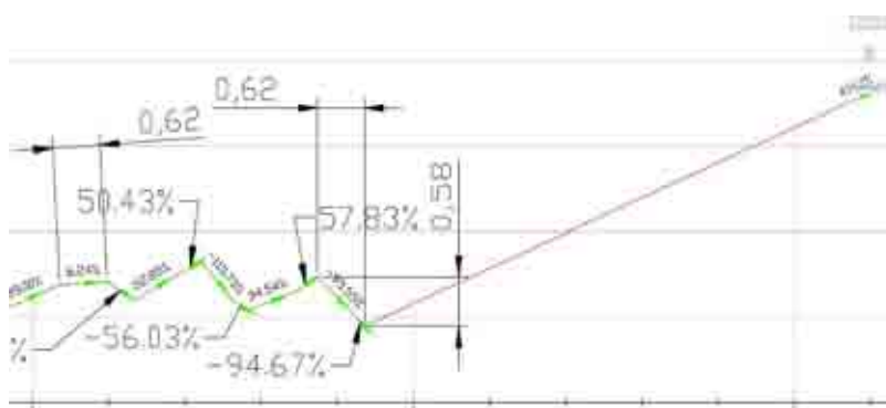
Figure 26 – Slopes of the surfaces shown on the transversal profile of the 3D surface model
