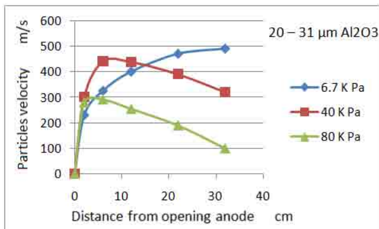
Figure 4 – Average velocities of \text{Al}_2\text{O}_3 particles with a granulation of 20-31 \mu\text{m} with the change of pressure
