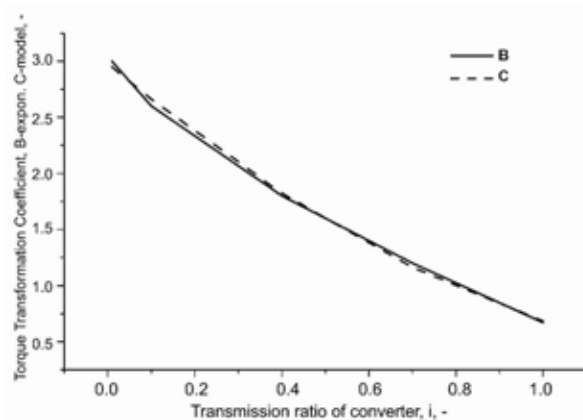
Figure 6 – Torque Transformation Coefficient
