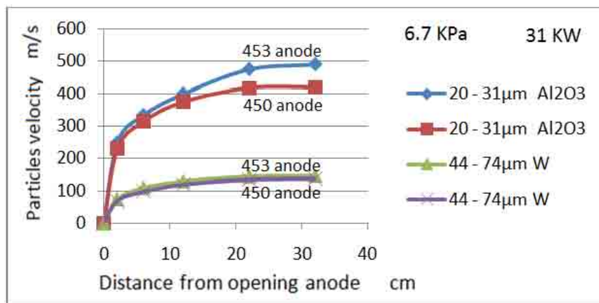
Figure 8 – Comparison of the average velocities of \text{Al}_2\text{O}_3 and W particles sprayed with 453 and 450 anodes at 6.7 KPa
