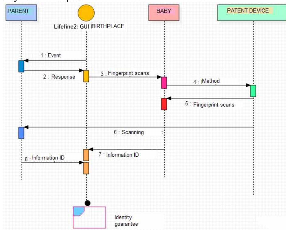
Figure 2 – Diagram of the information system sequences
