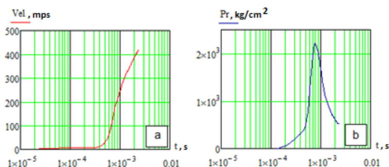
Figure 2 – Internal ballistic curves of the TT pistol (argument time): a – the projectile velocity in the barrel; b – internal ballistic curve of the mean pressure in the barrel.
