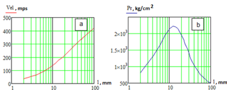
Figure 1 – Internal ballistic curves of the TT pistol (argument - bore length)
