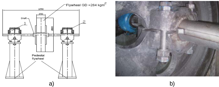
Figure 9 – Flywheel of a hydroelectric plant and its bearings
