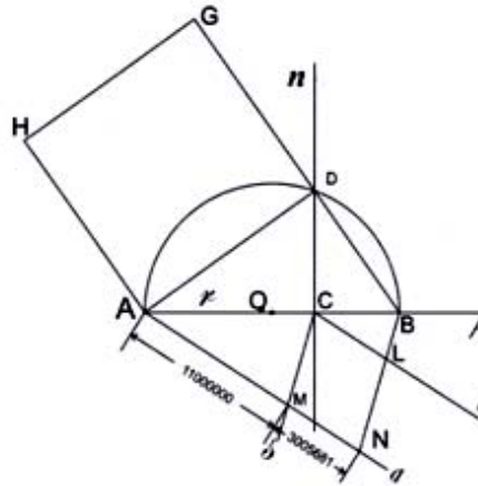
Figure 3 – Proportion of the lengths AC and CB in the ratio 11000000 : 3005681
