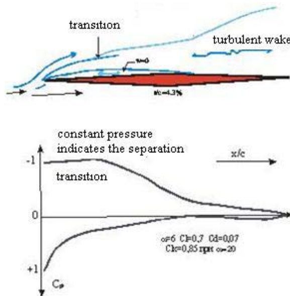
Figure 4 – Example of stalling a thin, sharp airfoil
