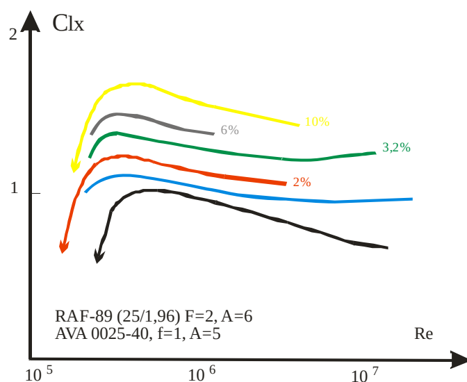
Figure 17 – Airfoil maximum lift, as a function of t/c , at Re = 4 \cdot 10^6
