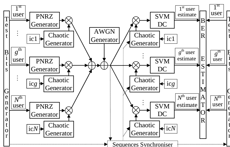
Figure 3 – Structure of the designed and implemented SVM CDMA system
