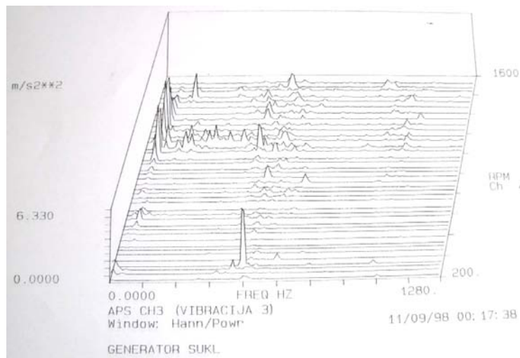
Figure 7 – Spectral map, Szz autospectrum, bearing L2
