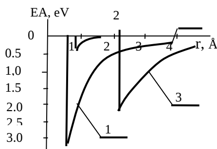
Figure 6 – Potential of the electron and molecule interaction: 1 - carbon, 2 – oxygen and 3 - titanium
