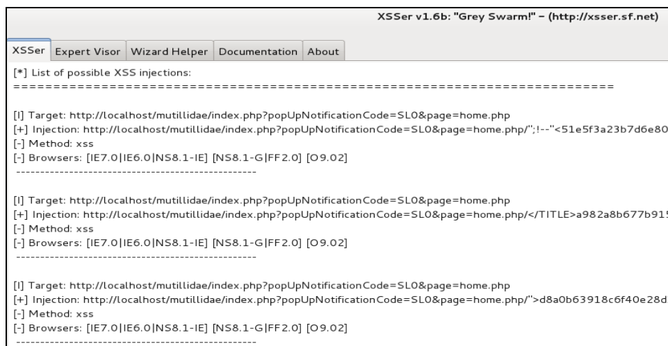
Figure 7 – XSSer – overview of a possible injection Рис. 7 – XSSer – отчет о возможных XSS инъекциях Slika – XSSer – prikaz mogućih XSS injekcija
