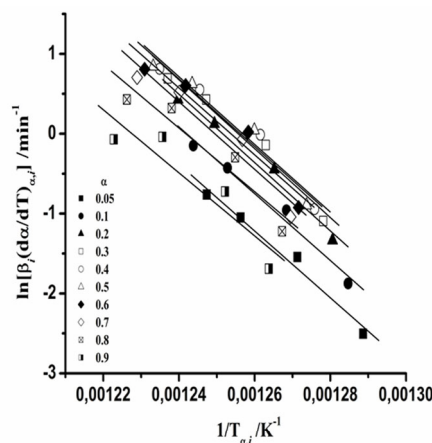
Figure 5 – The dependence of \ln[\beta_i(d\alpha/dT)_{\alpha,i}] versus (1/T_{\alpha,i}) at different values of \alpha , for the crystallization process of the amorphous \text{Fe}_{81}\text{B}_{13}\text{Si}_4\text{C}_2 alloy (full lines are the linear fitting (linearization) corresponding to different \alpha 's)
