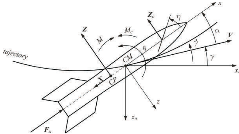
Figure 3 – Forces and moments acting on the missile
