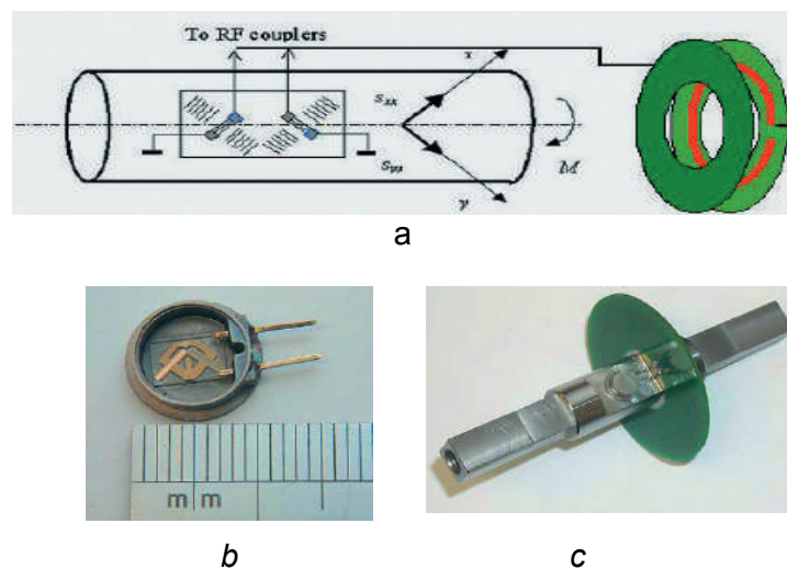
Slika 4 – Šematski prikaz (a) i fotografije PAT senzora (b) i (c) za merenje torzije Figure 4 – Schematic presentation (a) and photos of SAW sensors (b) and (c) for torsion measurements
