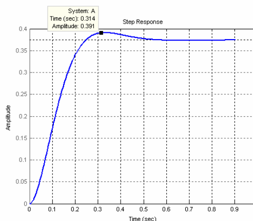
Slika 7 – Odziv motora dobijen simulacijom funkcije prenosa date izrazom (5) Figure 7 – Response of the DC motor simulated with the transfer function given by eq. (5)
