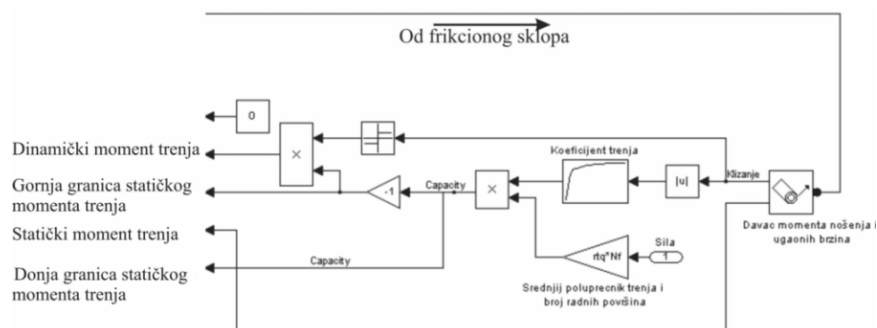
Slika 9 – Model trenja Figure 9 – Model of friction
