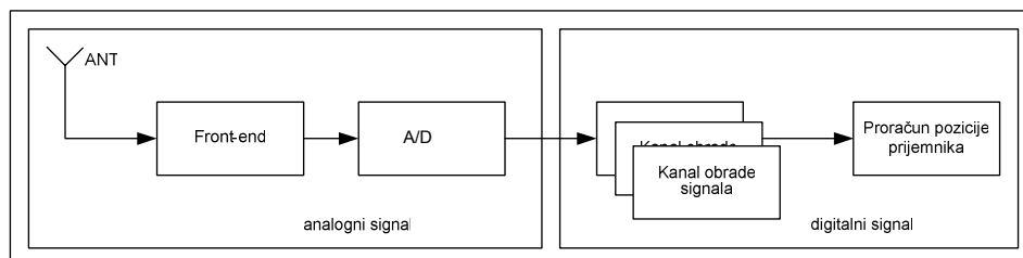
Slika 1– Blok šema softverskog prijemnika Figure 1 – Block diagram of software receivers
