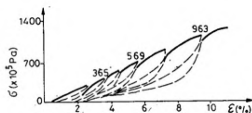
Sl. 11 — Promena \sigma(\varepsilon) i rasterećenje
