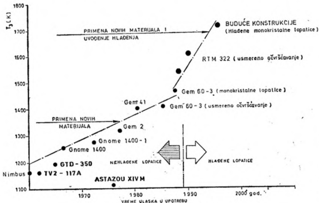
Sl. 4 — Trend rasta temperature ispred turbine ( T_3 ) GTR
