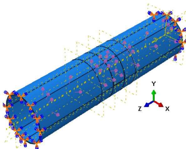
Figure 2 – Boundary condition of the corroded pipe
